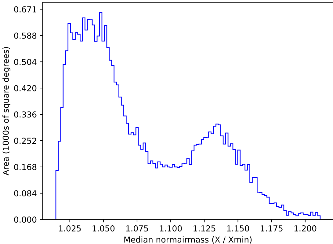
weather_cloudso2v3.4_10yrs All sky r band: Median normairmass
