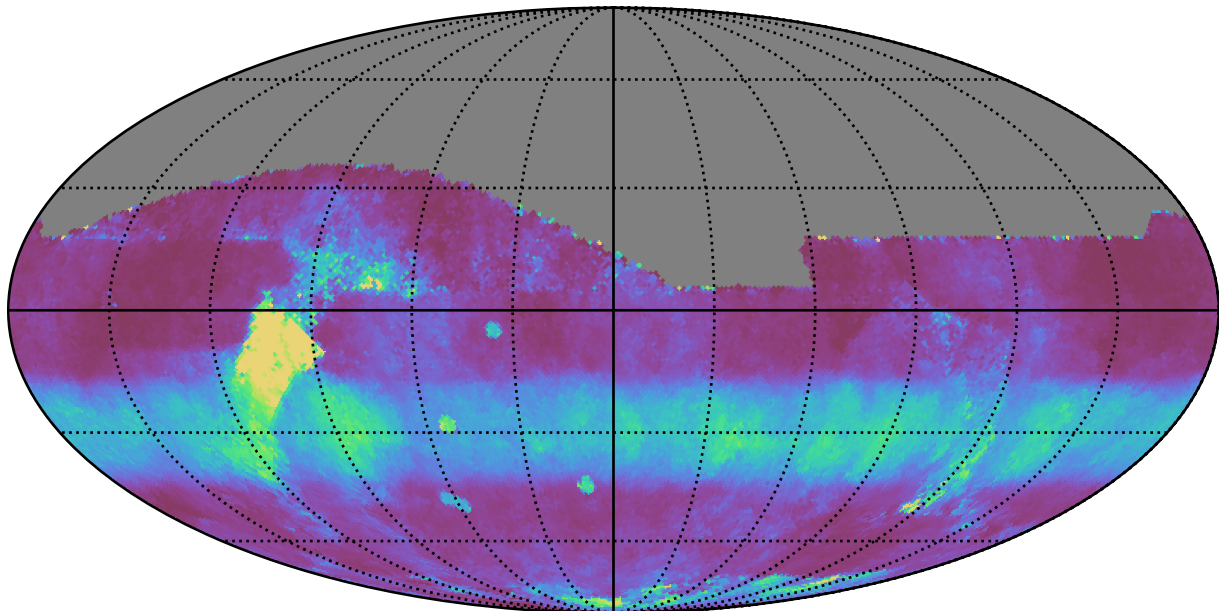
weather_cloudso2v3.4_10yrs All sky i band: Median normairmass
