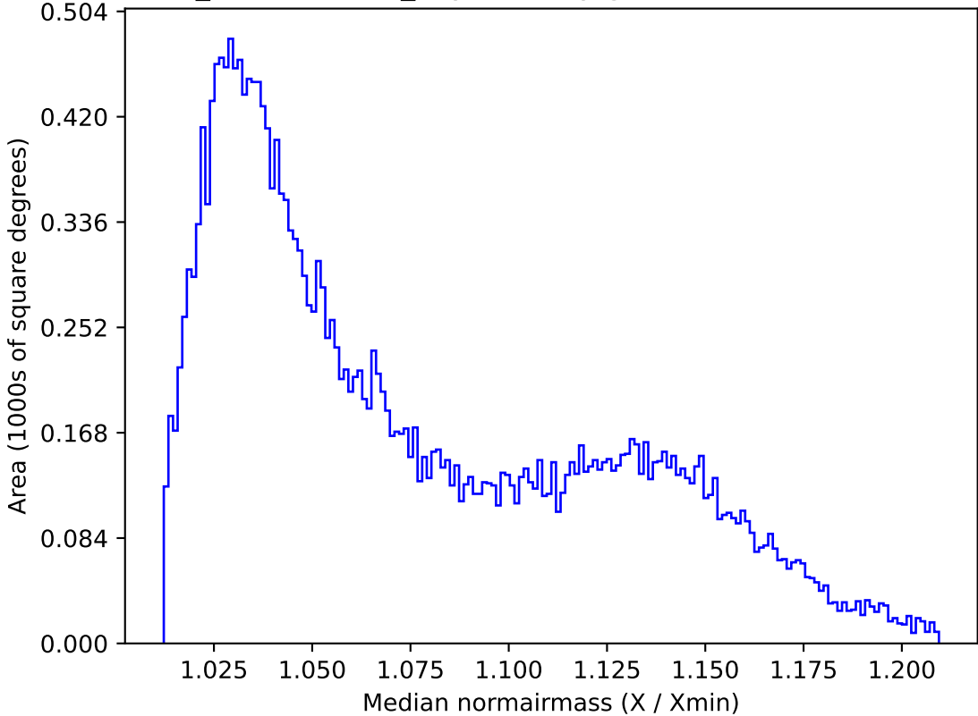
weather_cloudso2v3.4_10yrs All sky g band: Median normairmass
