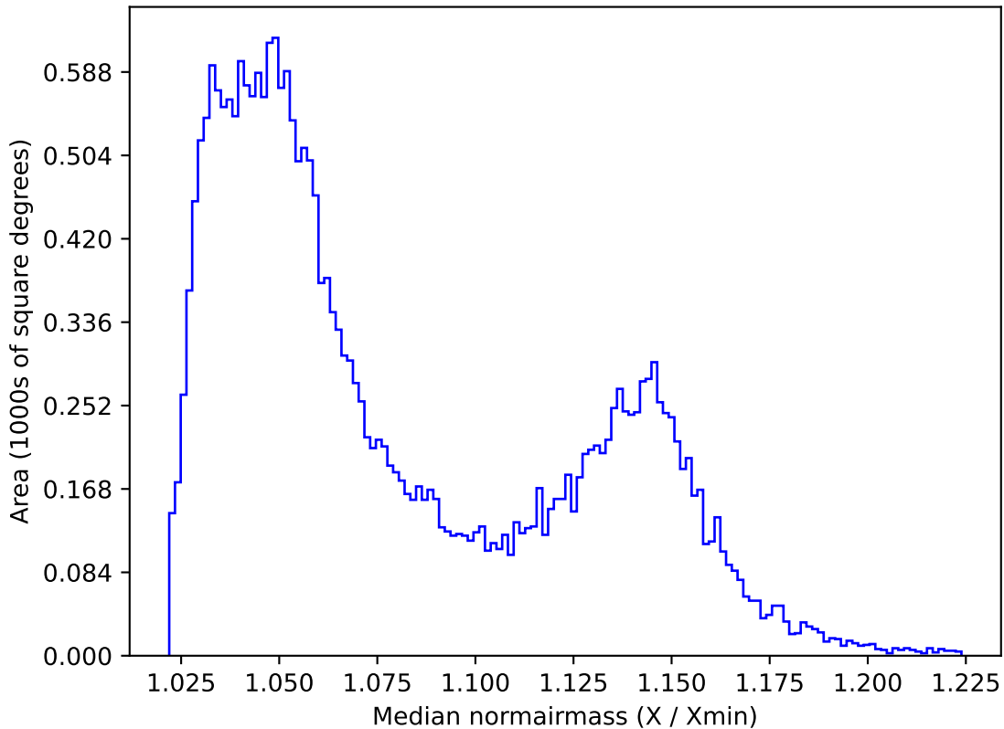
weather_cloudso2v3.4_10yrs All sky all bands: Median normairmass
