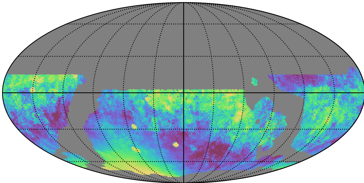
weather_cloudso2v3.4_10yrs WFD z band: Median moonDistance
