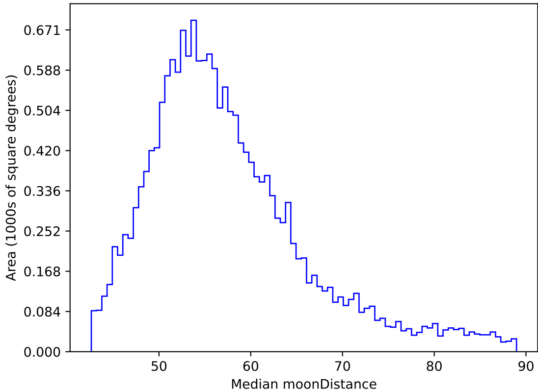
weather_cloudso2v3.4_10yrs WFD y band: Median moonDistance
