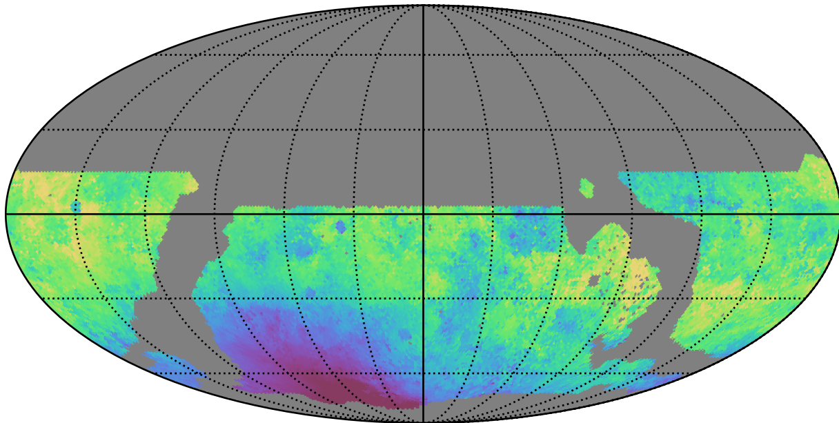
weather_cloudso2v3.4_10yrs WFD u band: Median moonDistance
