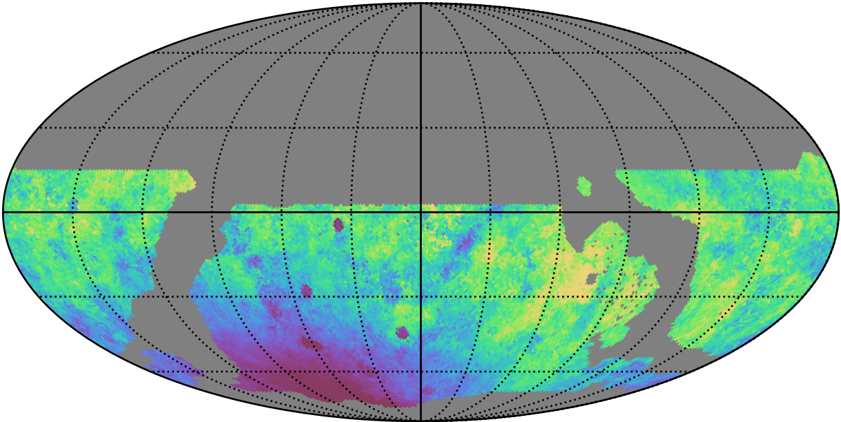
weather_cloudso2v3.4_10yrs WFD r band: Median moonDistance
