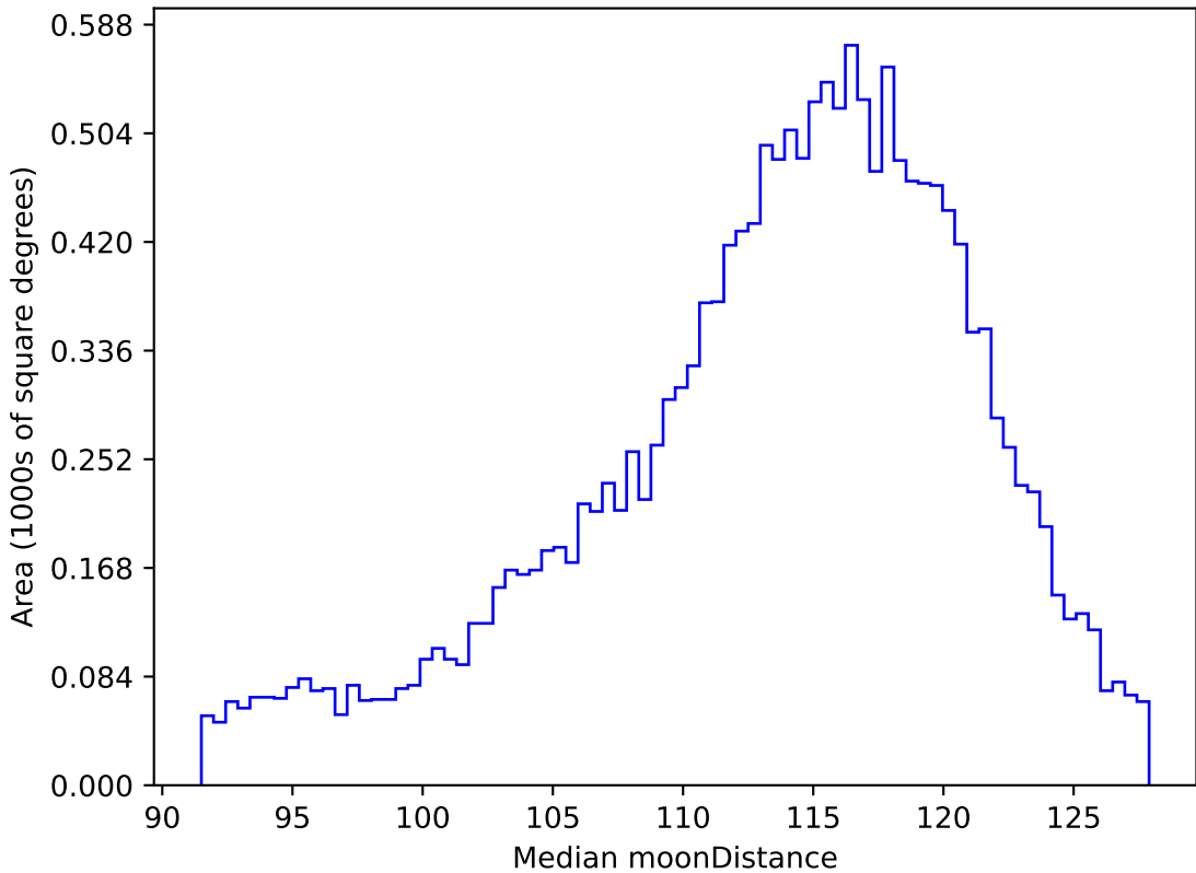
weather_cloudso2v3.4_10yrs WFD r band: Median moonDistance
