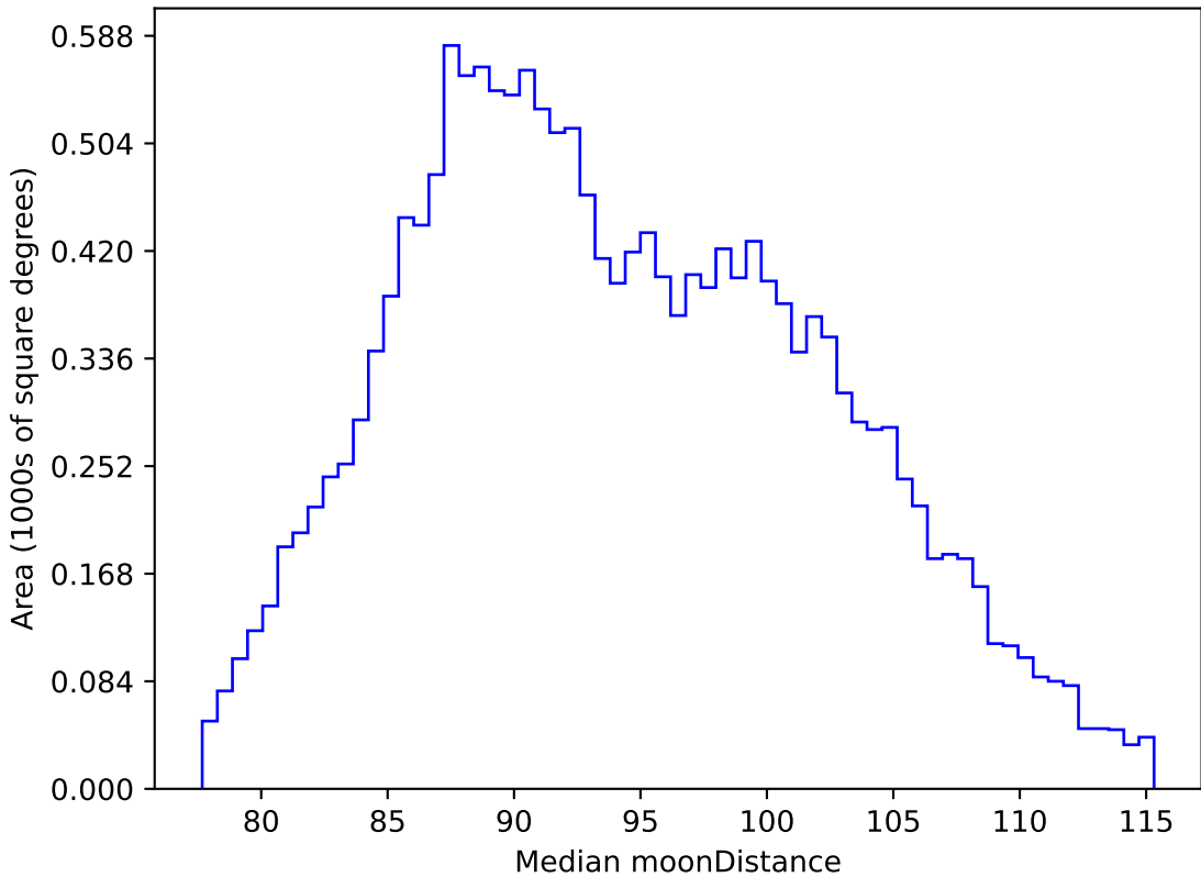
weather_cloudso2v3.4_10yrs WFD i band: Median moonDistance
