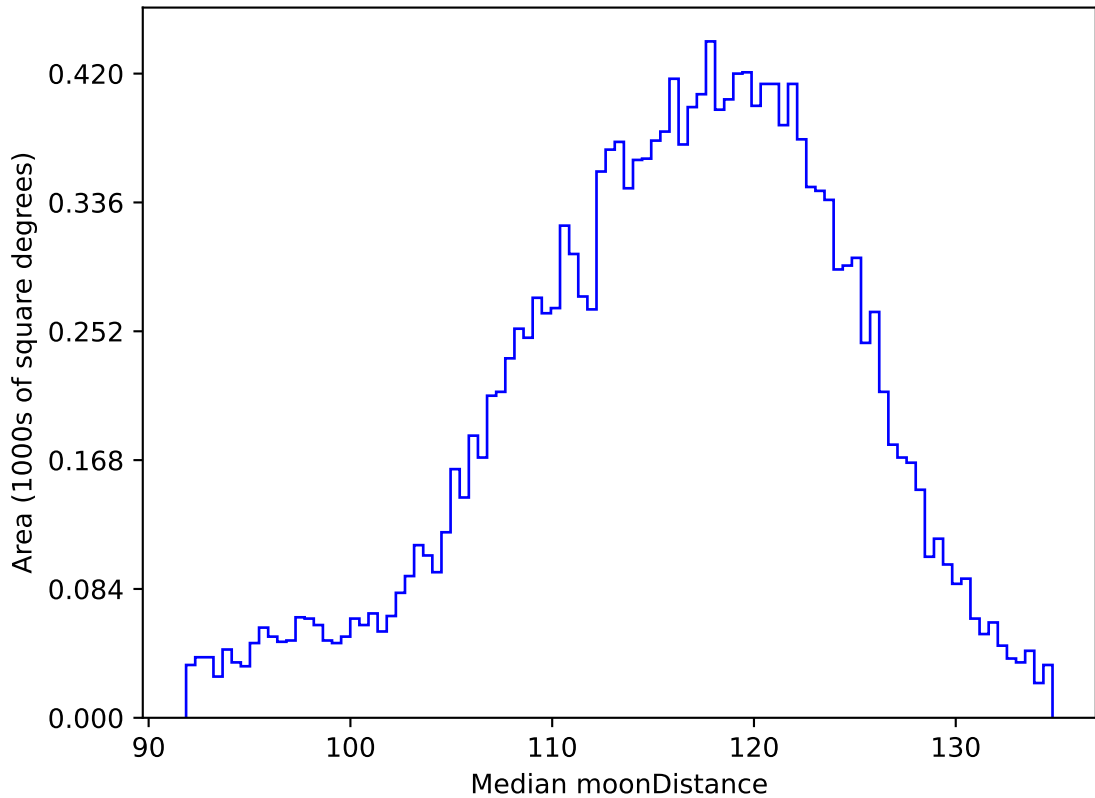
weather_cloudso2v3.4_10yrs WFD g band: Median moonDistance
