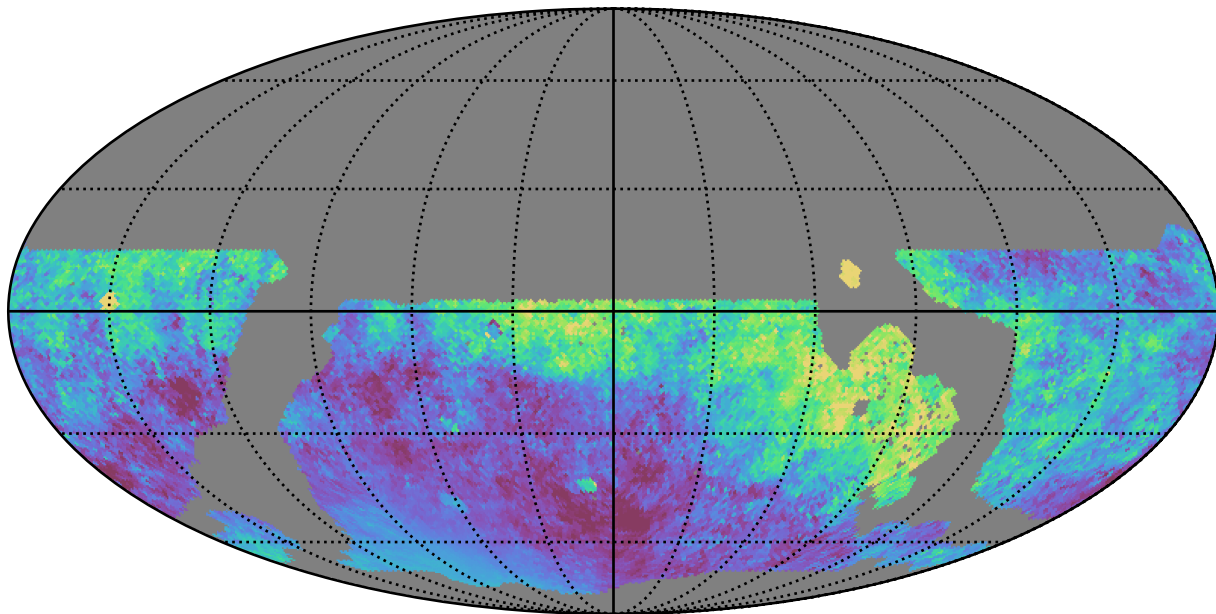
weather_cloudso2v3.4_10yrs WFD all bands: Median moonDistance
