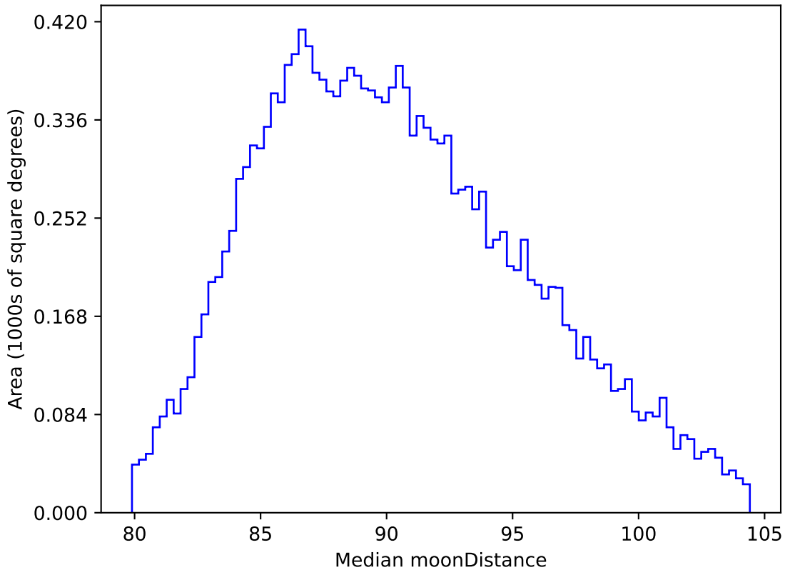
weather_cloudso2v3.4_10yrs WFD all bands: Median moonDistance
