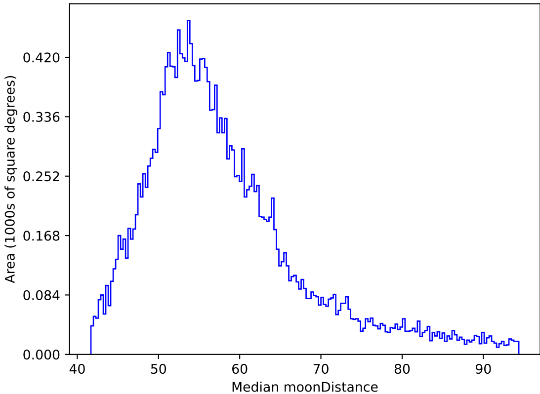
weather_cloudso2v3.4_10yrs All sky y band: Median moonDistance
