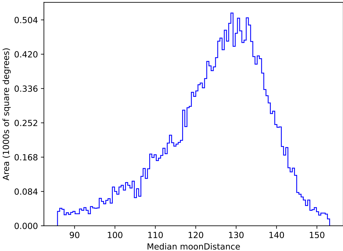
weather_cloudso2v3.4_10yrs All sky u band: Median moonDistance
