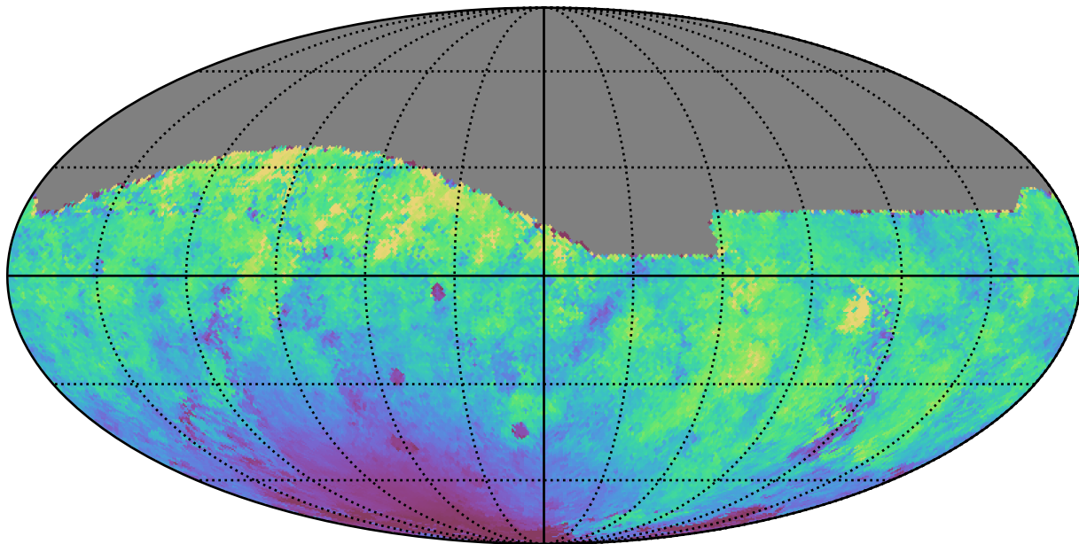
weather_cloudso2v3.4_10yrs All sky r band: Median moonDistance
