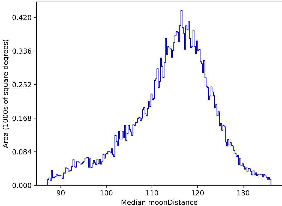
weather_cloudso2v3.4_10yrs All sky r band: Median moonDistance
