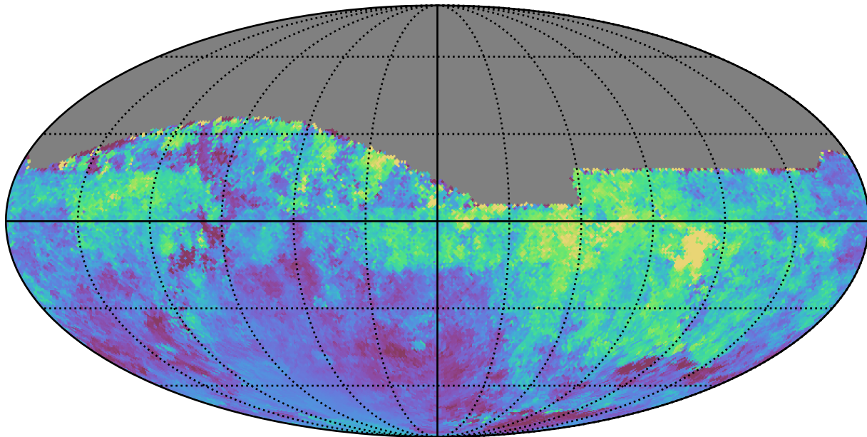
weather_cloudso2v3.4_10yrs All sky i band: Median moonDistance
