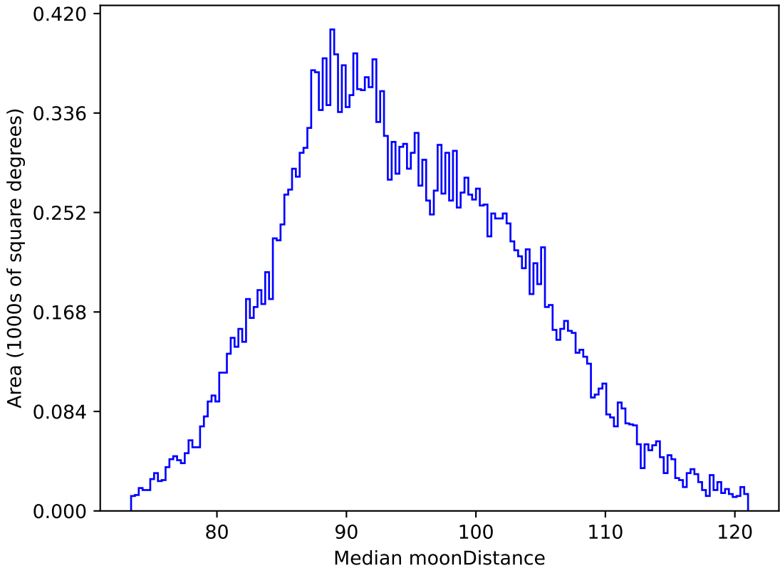
weather_cloudso2v3.4_10yrs All sky i band: Median moonDistance
