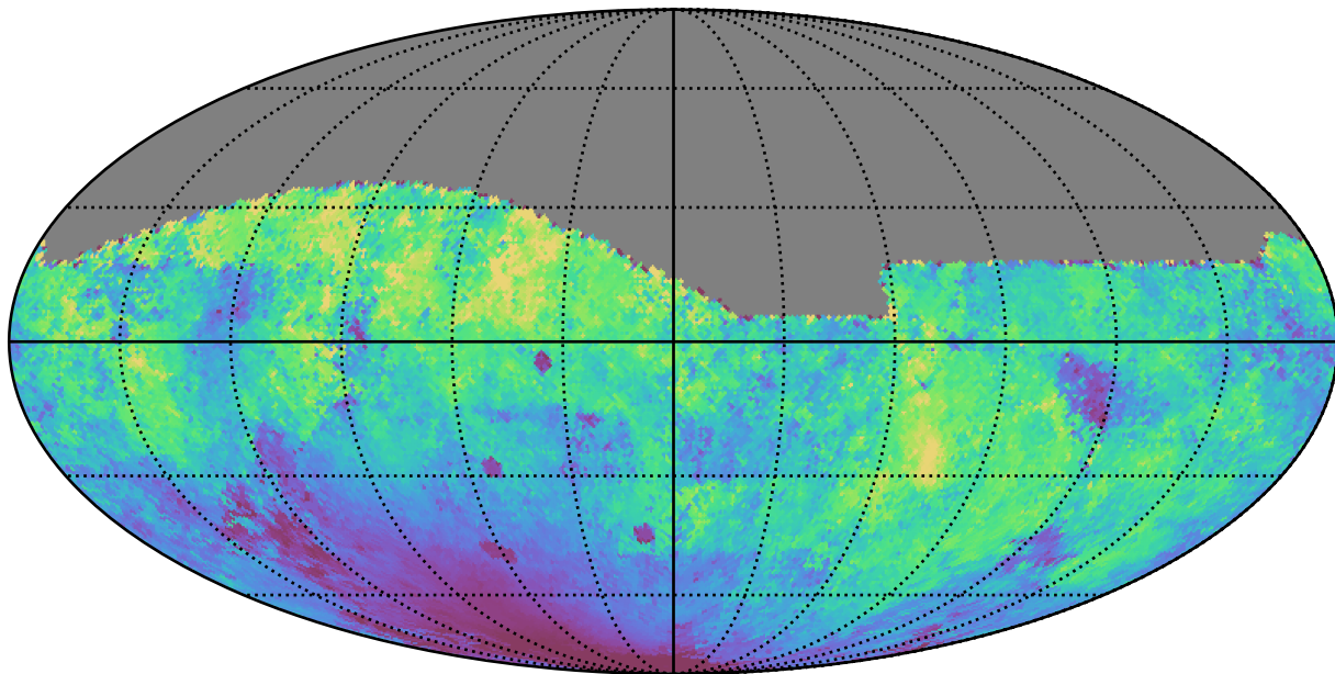
weather_cloudso2v3.4_10yrs All sky g band: Median moonDistance
