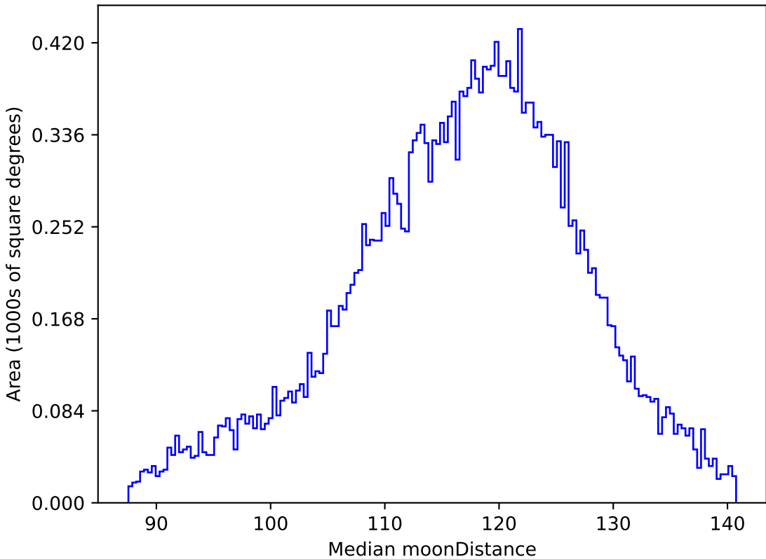
weather_cloudso2v3.4_10yrs All sky g band: Median moonDistance
