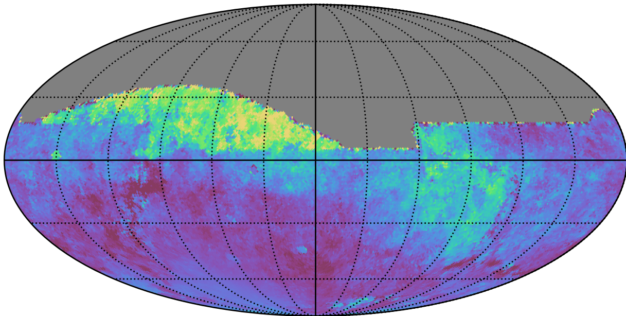
weather_cloudso2v3.4_10yrs All sky all bands: Median moonDistance
