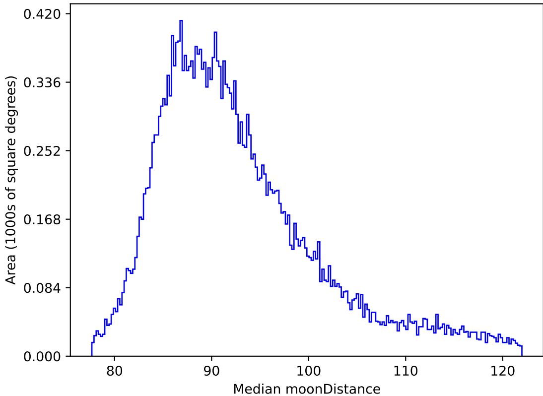
weather_cloudso2v3.4_10yrs All sky all bands: Median moonDistance
