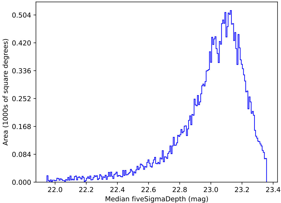
weather_cloudso2v3.4_10yrs Yr 1 z band: Median fiveSigmaDepth
