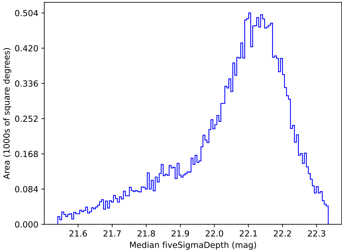
weather_cloudso2v3.4_10yrs Yr 1 y band: Median fiveSigmaDepth
