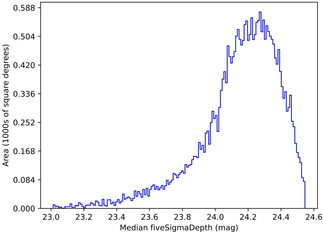
weather_cloudso2v3.4_10yrs Yr 1 r band: Median fiveSigmaDepth
