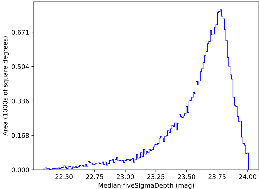
weather_cloudso2v3.4_10yrs Yr 1 i band: Median fiveSigmaDepth
