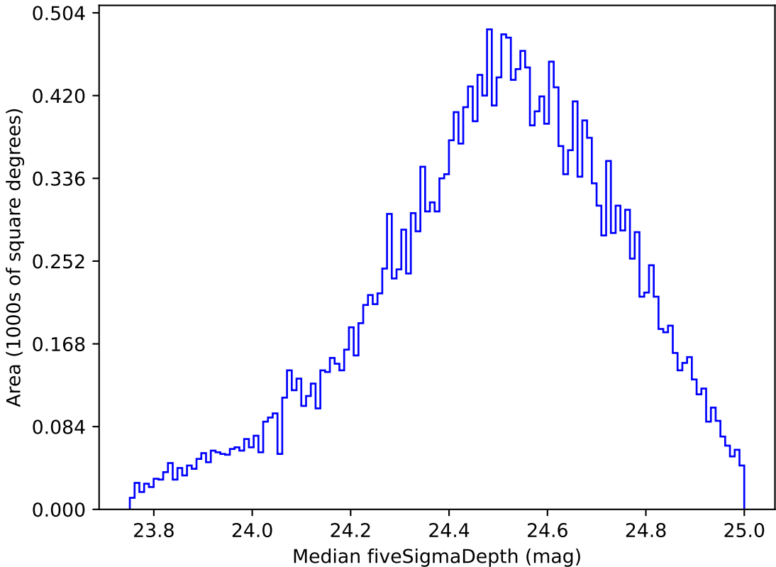
weather_cloudso2v3.4_10yrs Yr 1 g band: Median fiveSigmaDepth
