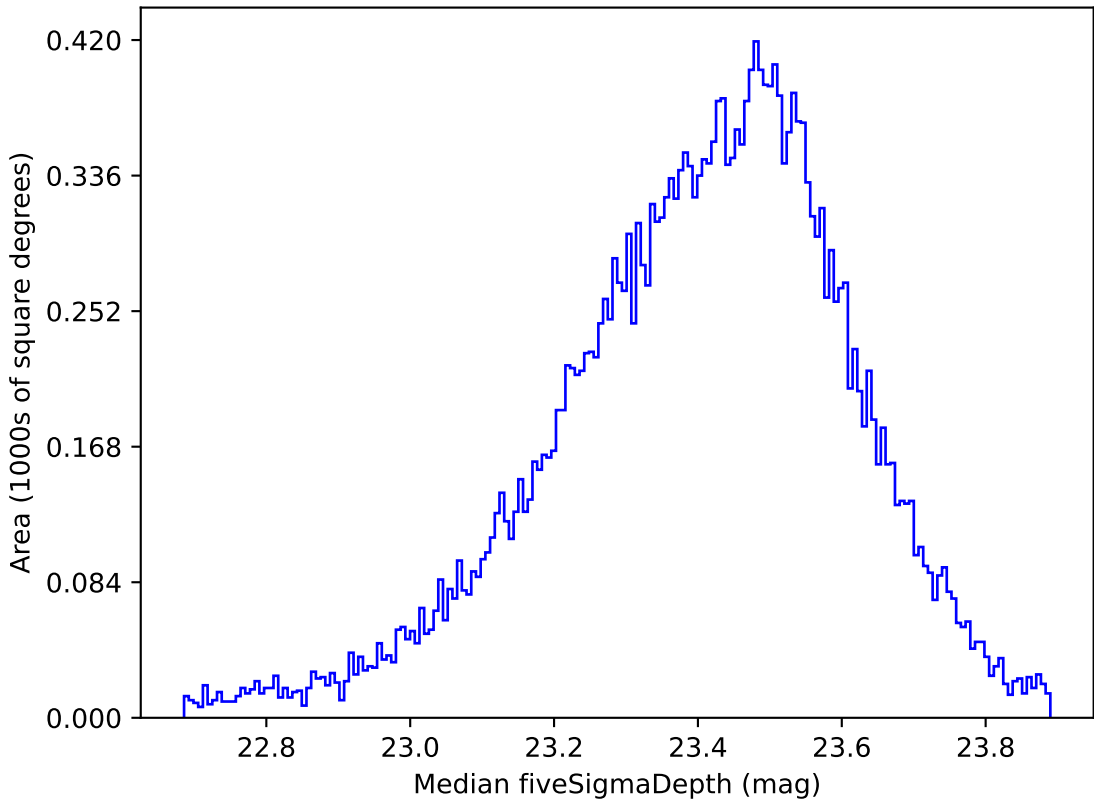
weather_cloudso2v3.4_10yrs Yr 1 all bands: Median fiveSigmaDepth
