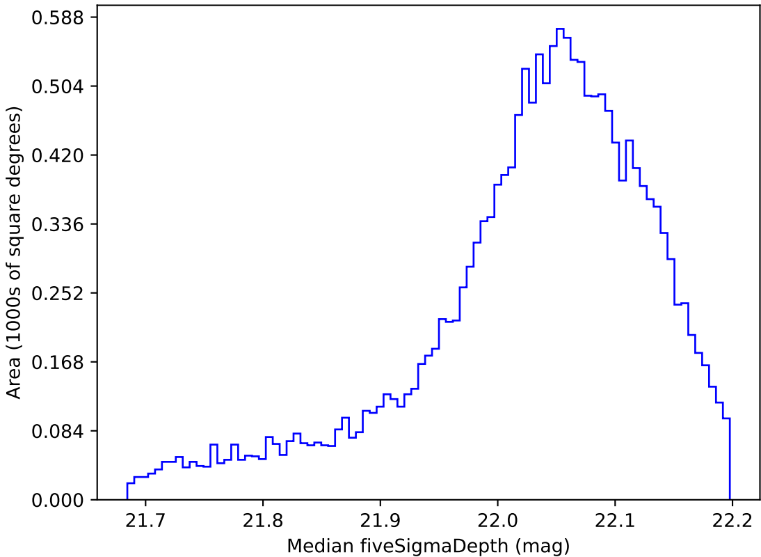
weather_cloudso2v3.4_10yrs WFD y band: Median fiveSigmaDepth
