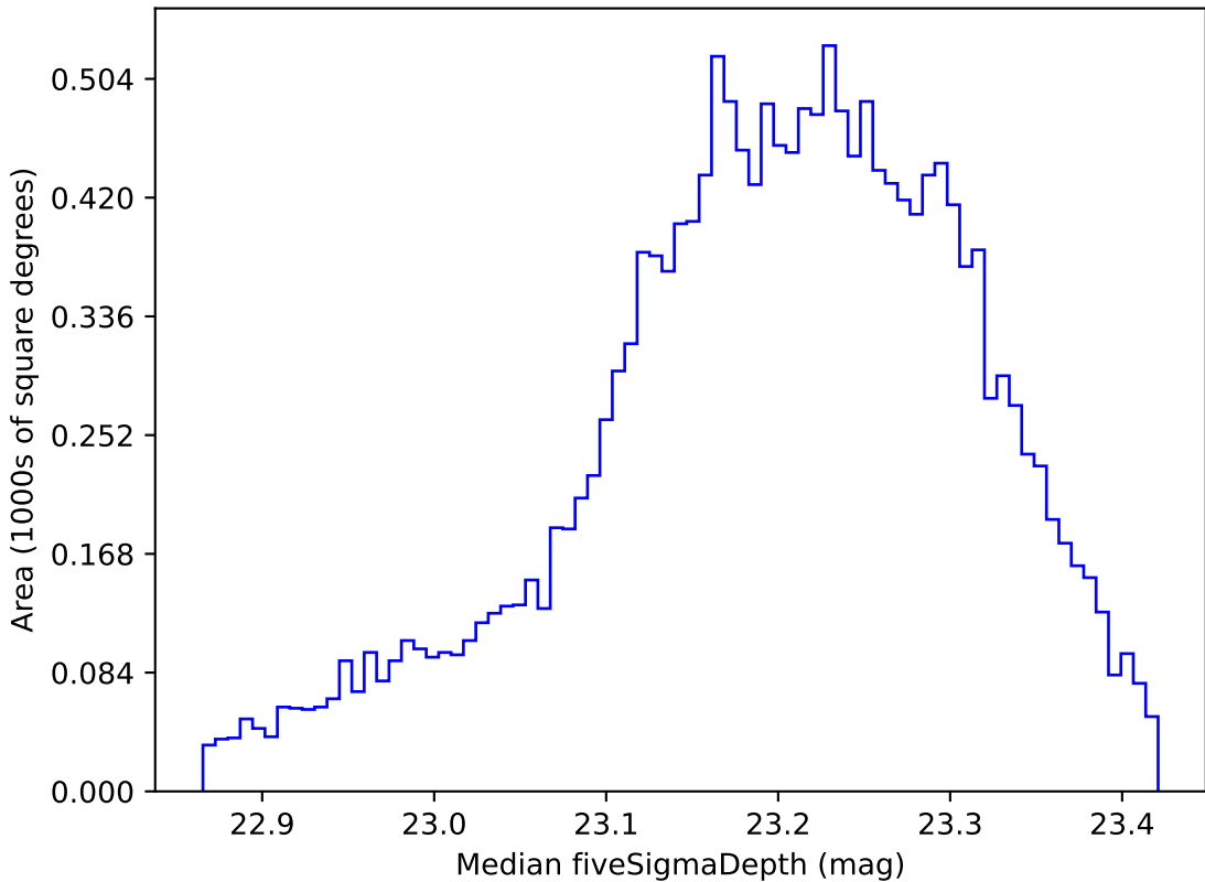
weather_cloudso2v3.4_10yrs WFD u band: Median fiveSigmaDepth
