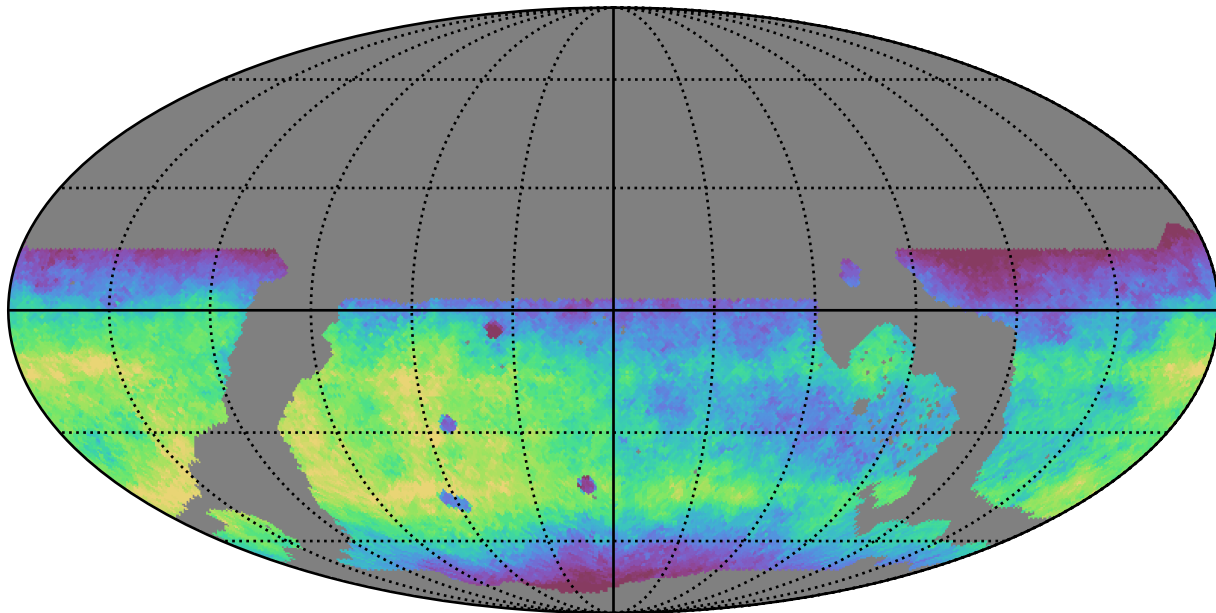
weather_cloudso2v3.4_10yrs WFD r band: Median fiveSigmaDepth
