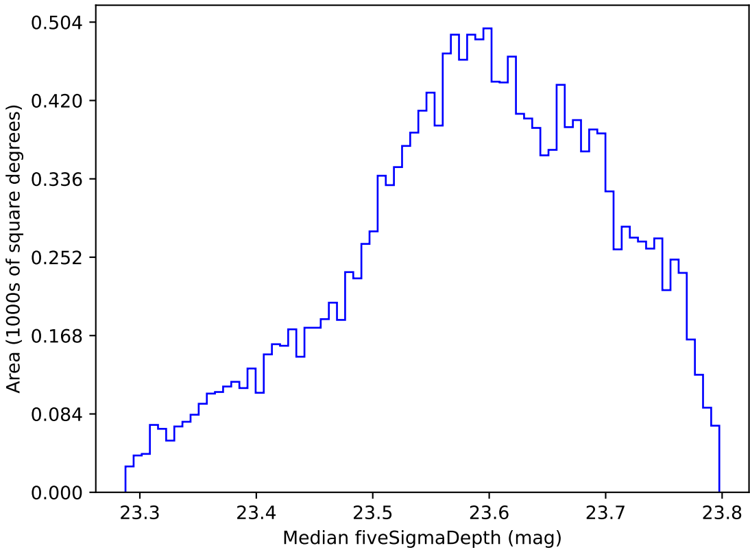
weather_cloudso2v3.4_10yrs WFD i band: Median fiveSigmaDepth
