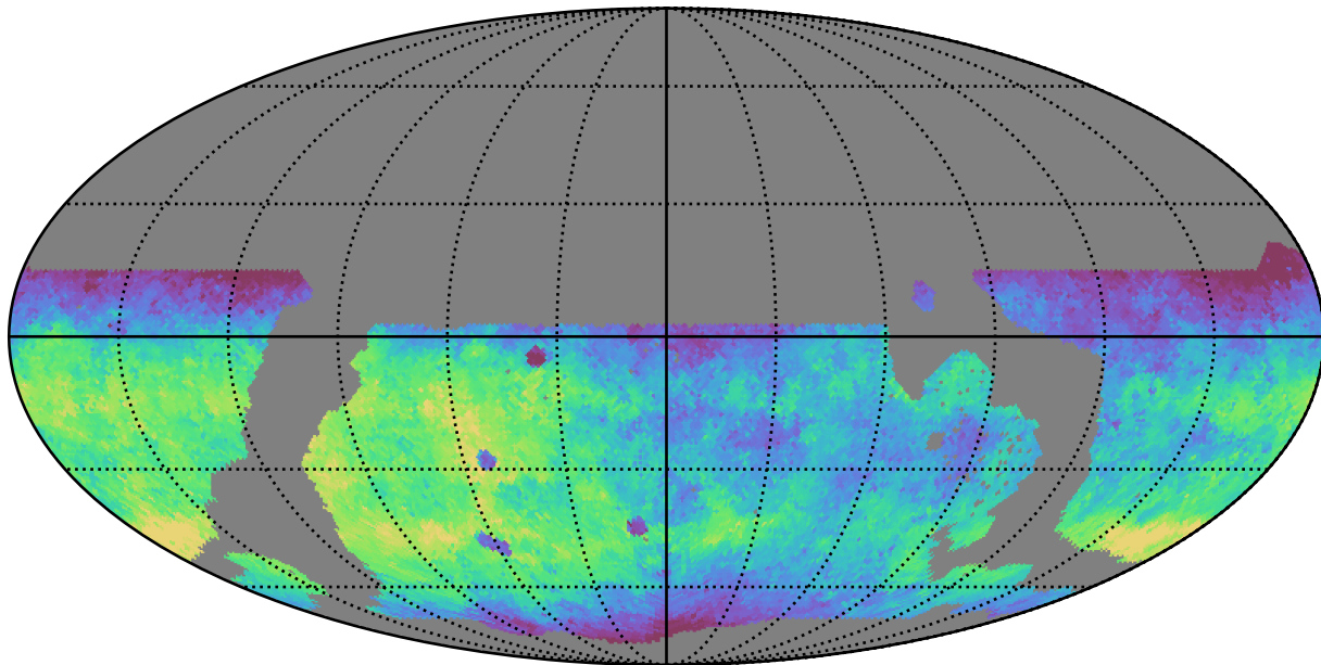
weather_cloudso2v3.4_10yrs WFD g band: Median fiveSigmaDepth
