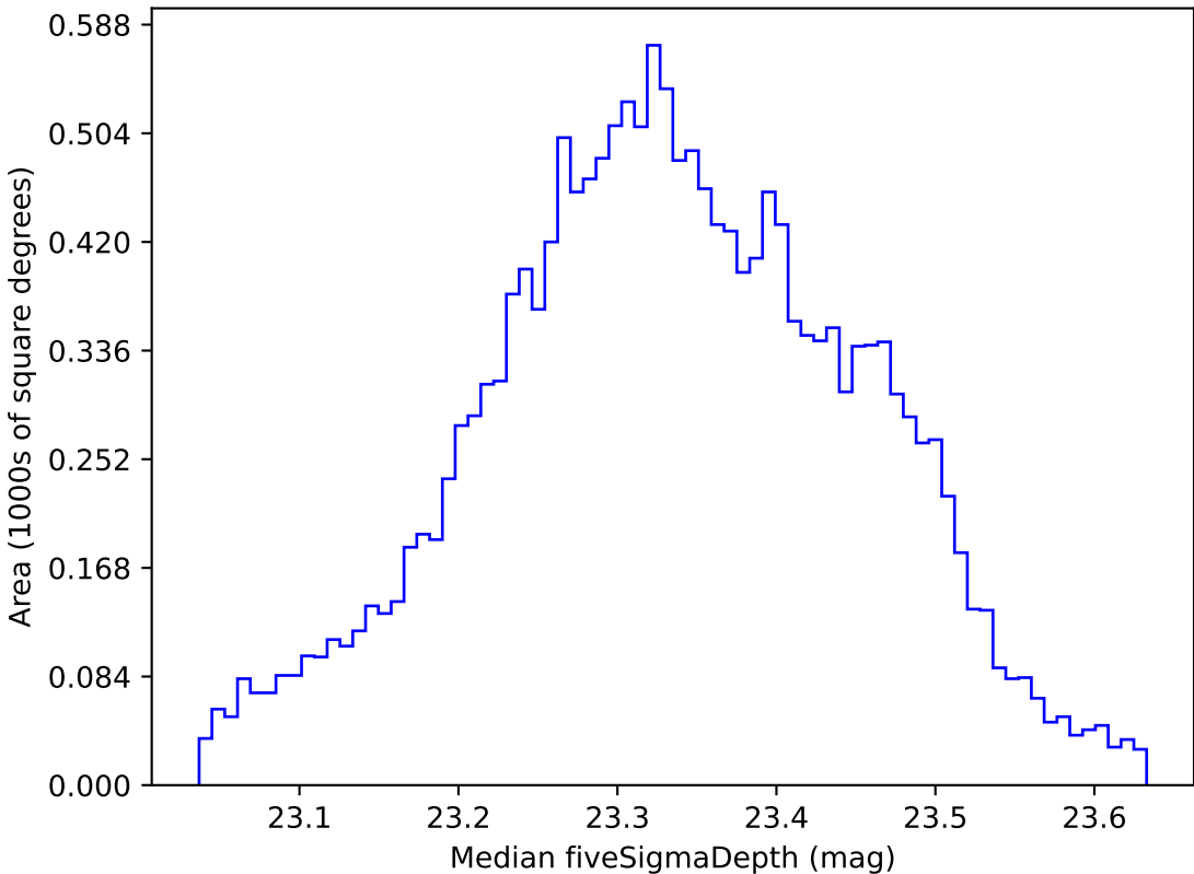
weather_cloudso2v3.4_10yrs WFD all bands: Median fiveSigmaDepth
