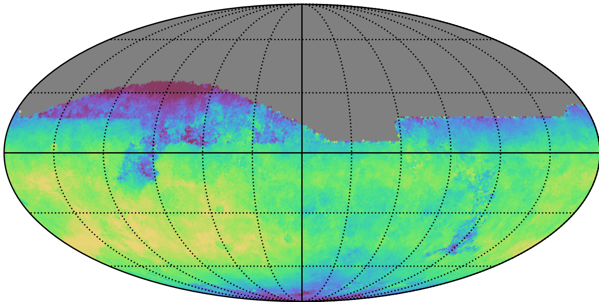
weather_cloudso2v3.4_10yrs All sky z band: Median fiveSigmaDepth
