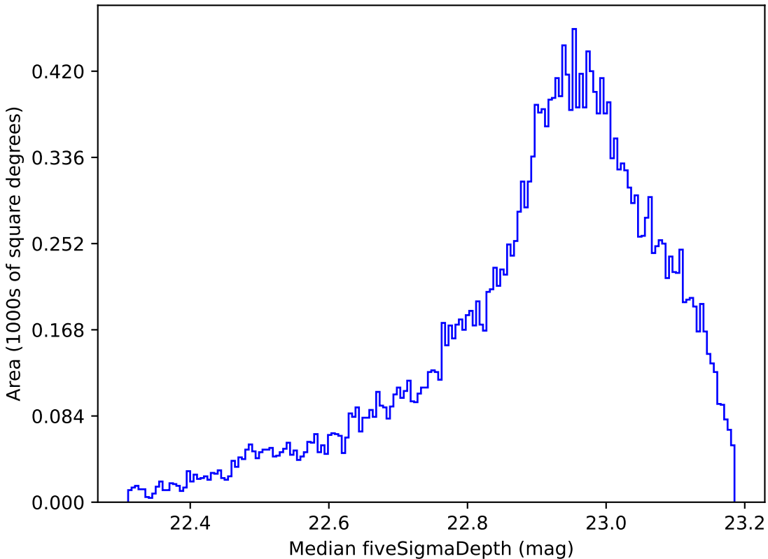
weather_cloudso2v3.4_10yrs All sky z band: Median fiveSigmaDepth
