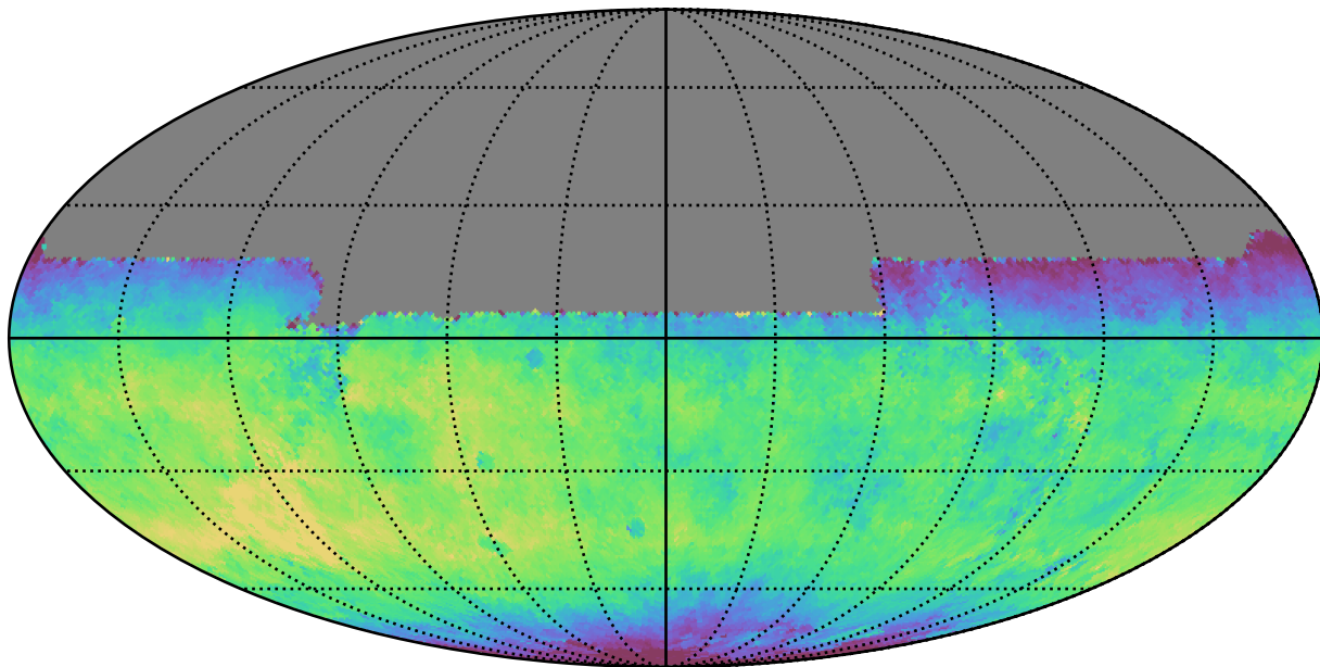
weather_cloudso2v3.4_10yrs All sky y band: Median fiveSigmaDepth
