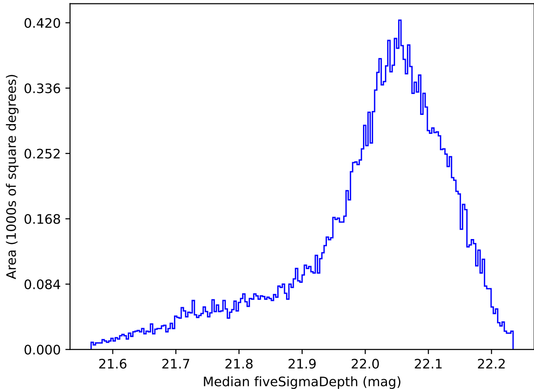
weather_cloudso2v3.4_10yrs All sky y band: Median fiveSigmaDepth
