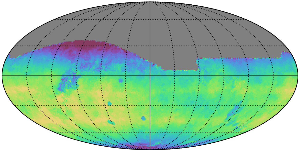
weather_cloudso2v3.4_10yrs All sky r band: Median fiveSigmaDepth
