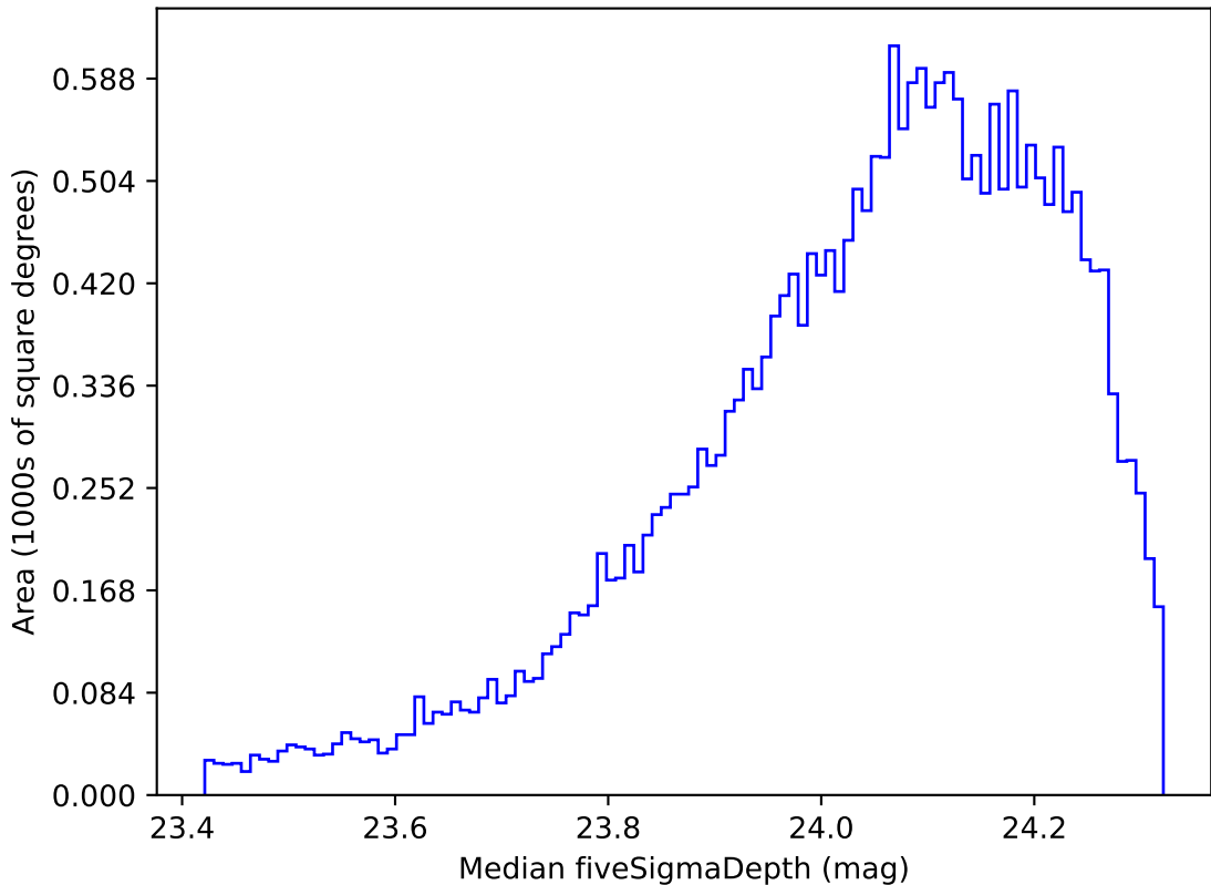
weather_cloudso2v3.4_10yrs All sky r band: Median fiveSigmaDepth
