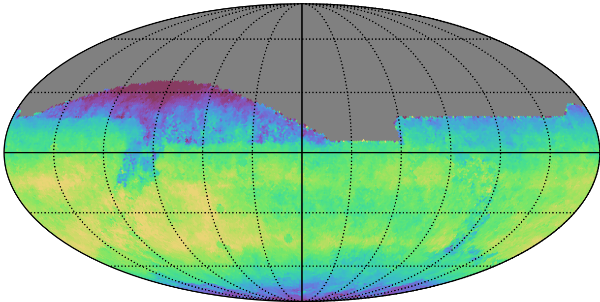
weather_cloudso2v3.4_10yrs All sky i band: Median fiveSigmaDepth
