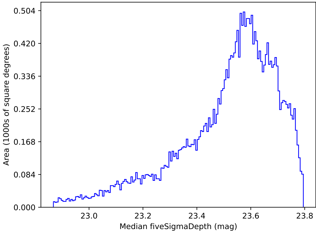
weather_cloudso2v3.4_10yrs All sky i band: Median fiveSigmaDepth
