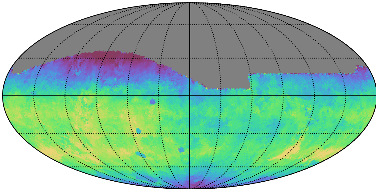
weather_cloudso2v3.4_10yrs All sky g band: Median fiveSigmaDepth
