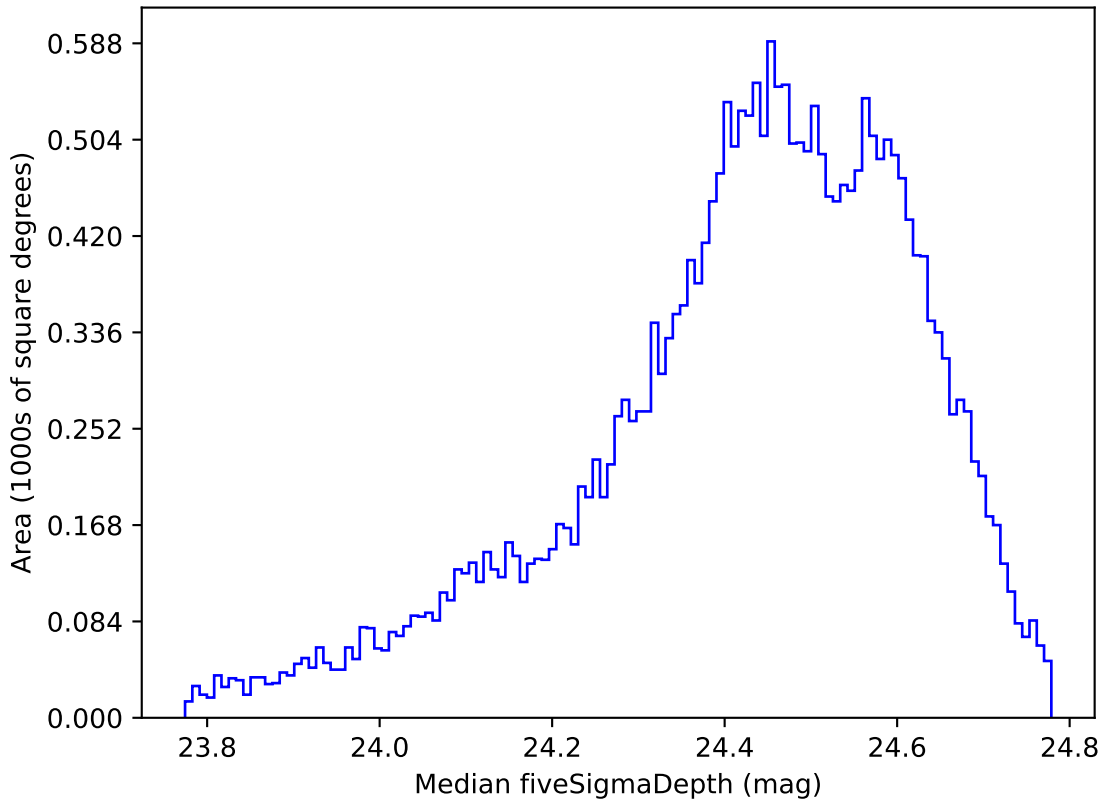
weather_cloudso2v3.4_10yrs All sky g band: Median fiveSigmaDepth
