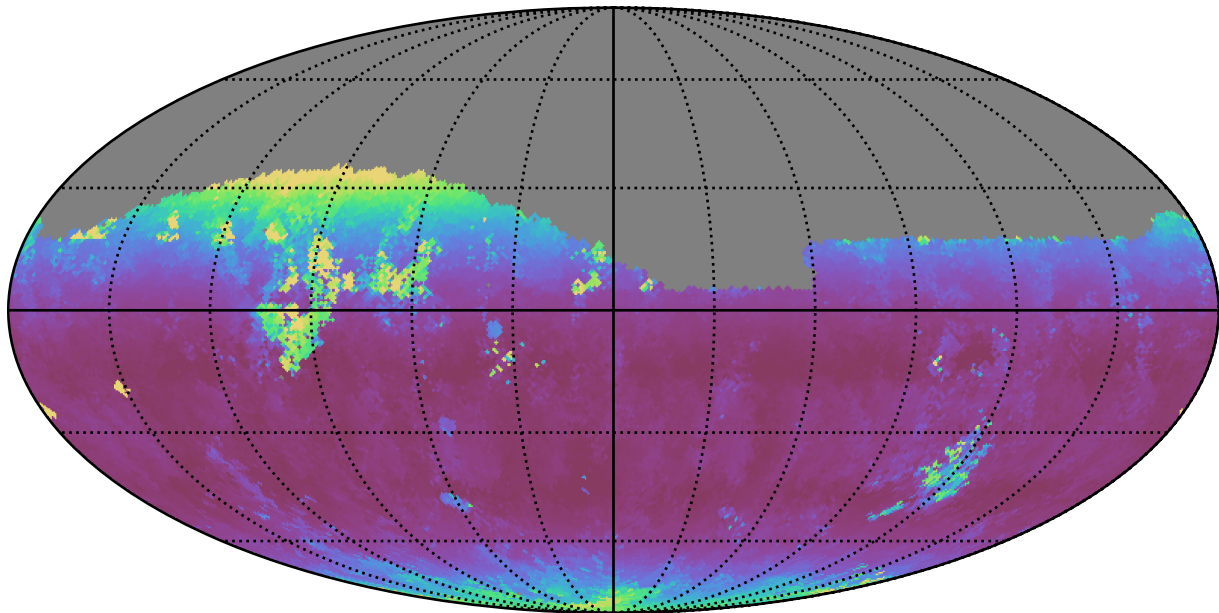
weather_cloudso2v3.4_10yrs Yr 1 z band: Median airmass
