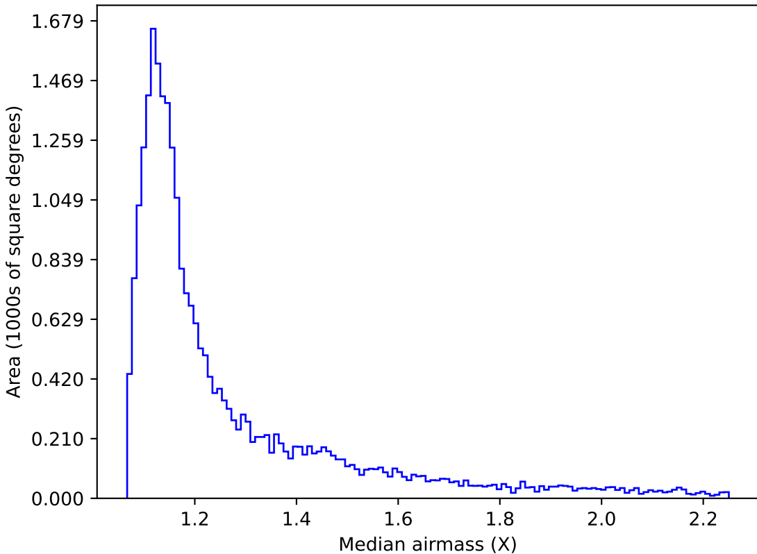
weather_cloudso2v3.4_10yrs Yr 1 z band: Median airmass
