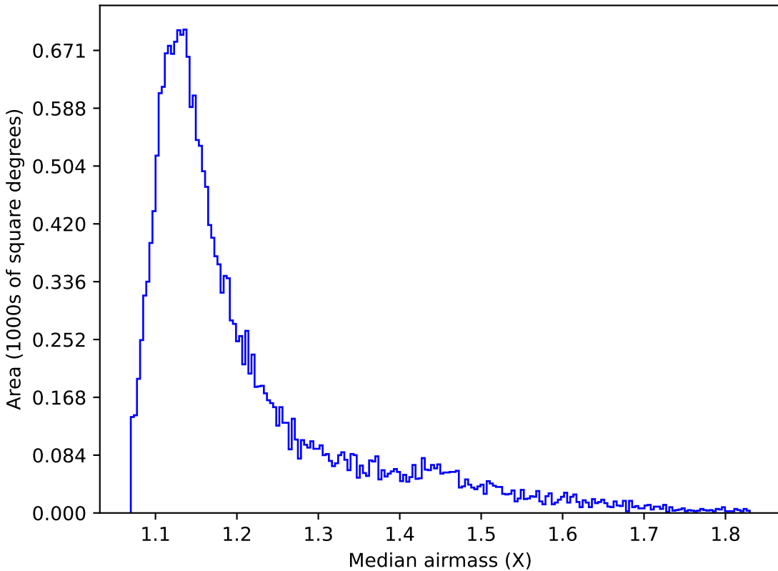
weather_cloudso2v3.4_10yrs Yr 1 y band: Median airmass
