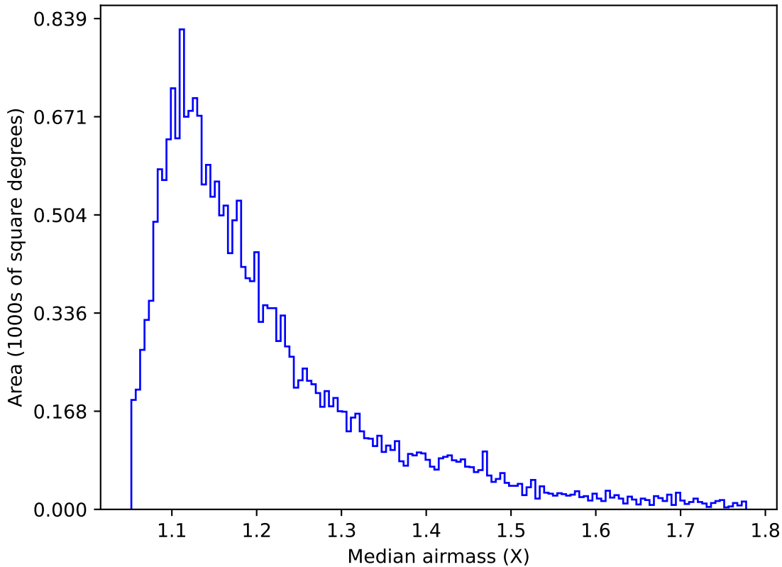
weather_cloudso2v3.4_10yrs Yr 1 u band: Median airmass
