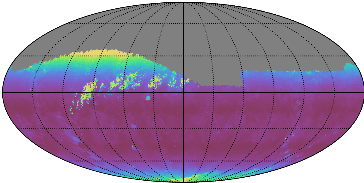
weather_cloudso2v3.4_10yrs Yr 1 r band: Median airmass
